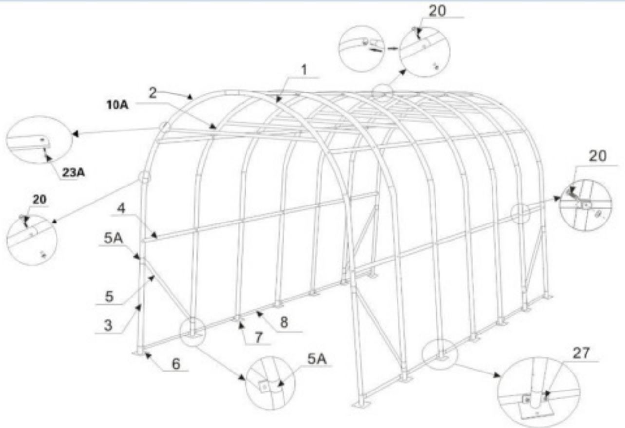
Figure 4 W4.3 xL9.2 x H4.3m
